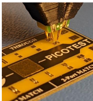
Fig. 13 - P2102A 2-port Thru-Calibration with Bode 100.
