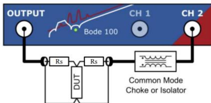
Fig. 4 - 2-port Shunt-Thru with series resistance impedance measurement setup using Bode 100 and Picotest ground isolator J2102B.
