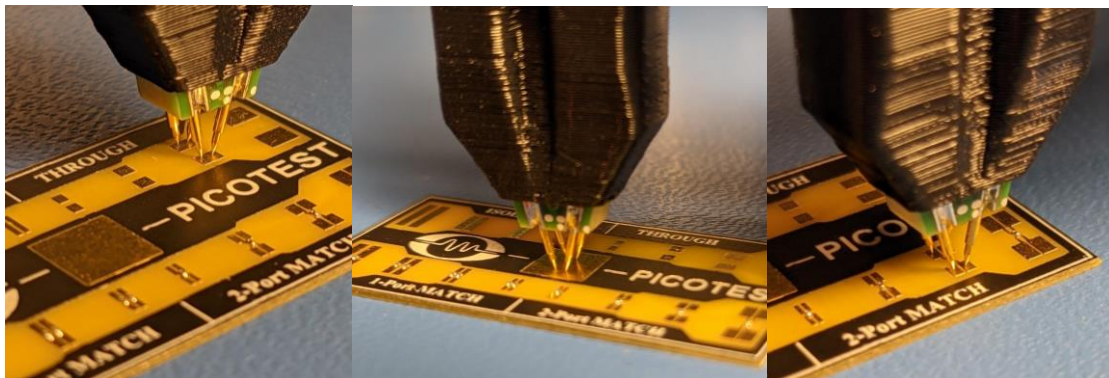
Fig. 12 - P2102A 2-port Calibration Open (left), Short (center), and Load (right) with Bode 100.
